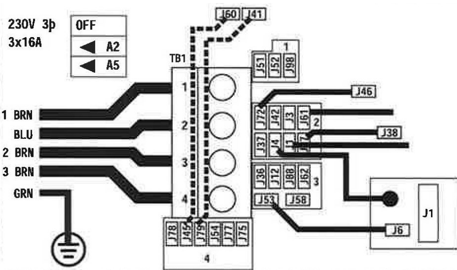
SRBP2100X Spa Pack - 3-Service
