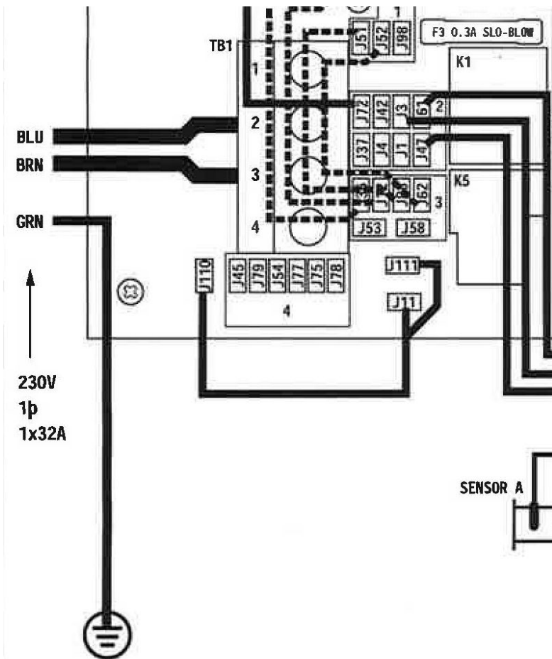
SRBP2100X Spa Pack – Single Service
